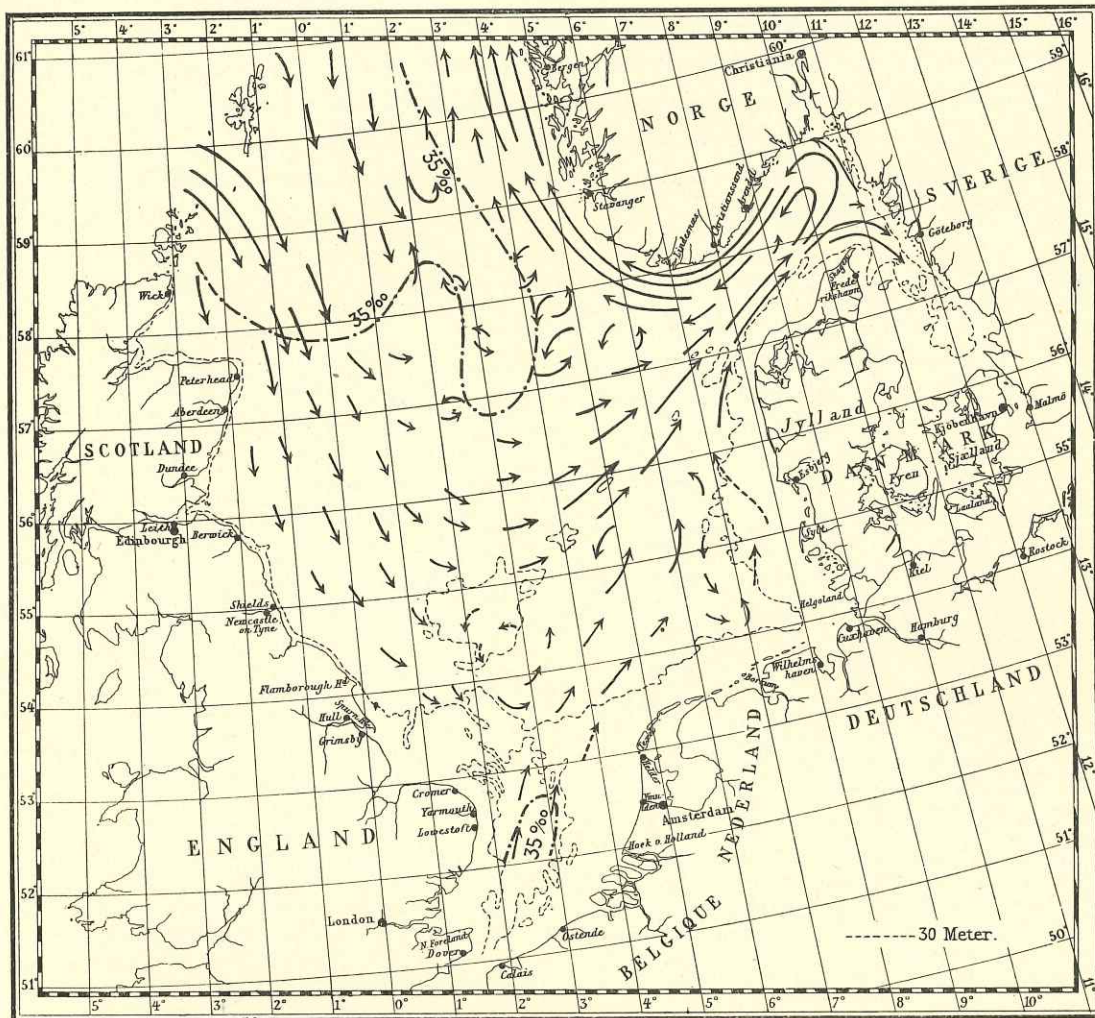
Fig. 5. The direction of the resulting Currents at ca. 30 meters depth in the North Sea and the Skagerrak. Drawn up by AAGE J. C. JENSEN on the basis of publications of WEMYSS FULTON, C. H. BROWN, G. P. BIDDER, G. BÖHNECKE, A. SCHUMACHER, H. KELLER, M. KNUDSEN, M. KNUDSEN and KIRSTINE SMITH, J. GEHRKE, O. PETERSSON, ROSENDAAL and WIND, VAN EVERDINGEN and WIND, etc.
