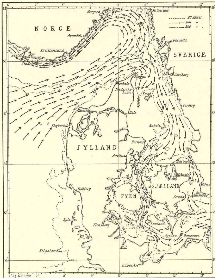
Fig. 6. The direction of the resulting Currents in the intermediate layers (ca. 30—100 m) of the Skagerrak and the lower layers of the Kattegat and Belt Sea. Drawn up by AAGE J. C. JENSEN on the basis of observations of O. PETERSSON, G. EKMAN, MARTIN KNUDSEN, J. P. JACOBSEN, RUPPIN etc.
