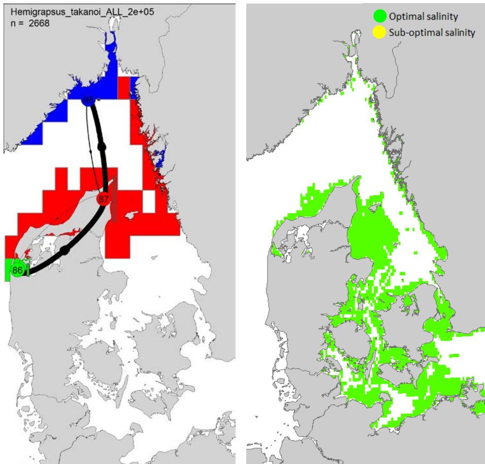
Figure 19. Left: Hydrographic regions identified for Hemigras tankoi based on 3 years larval dispersal simulation (2005, 2010 and 2012). Right: Predicted habitat based on substrate preferences and salinity tolerance of adult life stages. For detailed description on how to read figures, see methodology section in this appendix.
