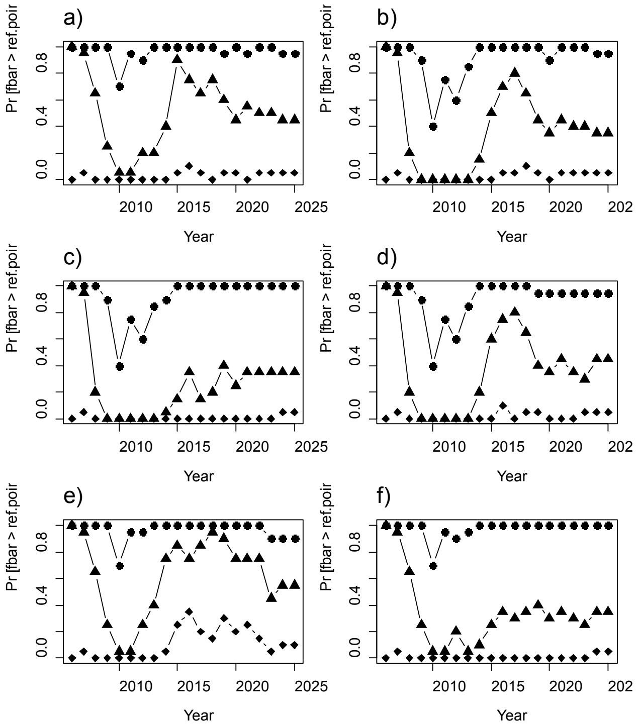
Figure 43. Probabilities to be above some reference levels of West cod fishing mortality F_{bar}(3-6) for 6 selected scenarios a) to f) corresponding to scenarios 1, 2, 5, 6, 7, 8 (see Table 14). circle: F(3-6) > 0.3 ; triangle: F(3-6) > 0.6 ; diamond: F(3-6) > 1.0
