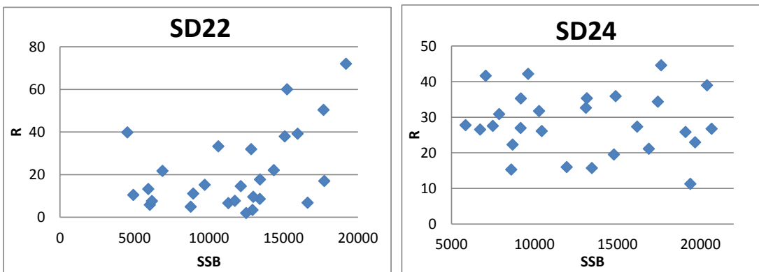
Figure 22. Stock-recruitment relationship from separate assessments for SD22 and SD24.
