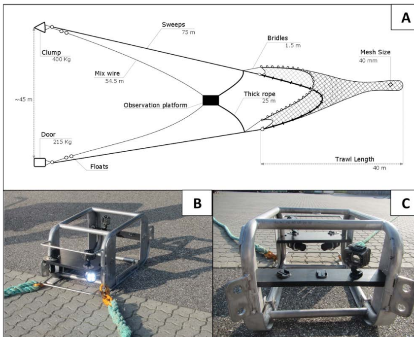
Figure 8. A) FLEXSELECT and position of observation platform. B) Observation platform with scaring lines (back view). C) Observation platform, front view.
