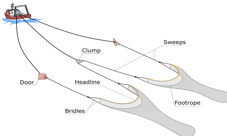
Figure 2. Schematic illustration of the trawl design and twin-rig configuration used by the Danish Nephrops -directed mixed trawl fishery.
