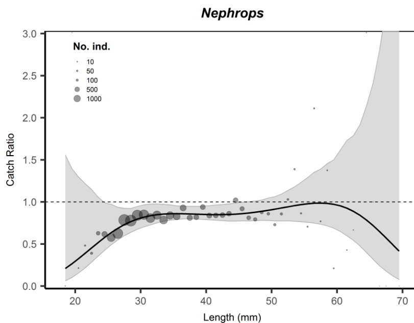
Figure 10. Catch ratio for the target species Nephrops . The curve (solid line) represents the modelled catch ratio fitted to the experimental points (dots). The size of the dots is relative to the total number of individuals of that length class caught in either trawl. Experimental points above 3.0 in Catch Ratio were placed at the upper margin of the plot. The grey ribbon represents 95% Efron Confidence Intervals. The dashed horizontal line, located at 1.0, describes equivalence in catch between the two trawls.
