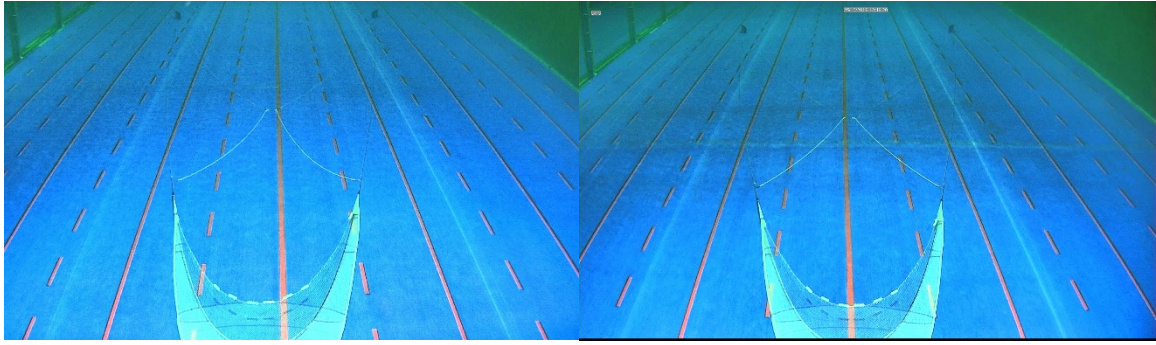
Figure 19. Pictures from the scaled model of FLEXSELECT in SINTEF's trawl tank in Hirtshals, showing the device at two different spread openings. On the left, with smaller doors spread the scaring lines are not in tension and can sweep the seafloor. On the right, at a greater spread the scaring lines are in tension and may rise above the seafloor; some oscillation in the lines in proximity of the wings tip was also observed (not shown in figure).
