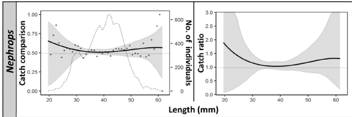
Figure 5. Catch comparison rates and catch ratios for the target species Nephrops . Left panel: the curve (solid line) represents the modeled catch efficiency fitted to the experimental points (dots). The grey band represents 95% confidence intervals and the dashed line the length distribution observed in the catch. The dotted horizontal line, located at 0.49, describes equivalence in catch rates between the two trawls. Right panel: catch ratio curve (solid line) with 95% confidence intervals (grey band). The dotted horizontal line, located at 0.98, describes equivalence in catch rates between the two trawls.
