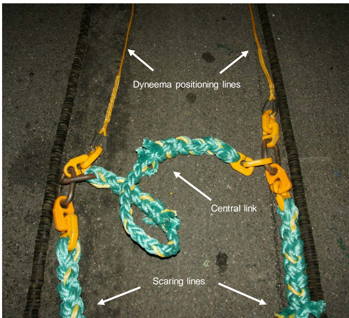
Figure 14. Different components of the commercial version of FLEXSELECT used on FN 436 Tove Kajgaard.
