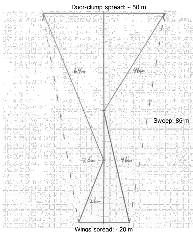
Figure 13. Schematic illustration of the two geometries of FLEXSELECT tested. The left part of the scheme illustrates the configuration with short scaring lines (26 m), while the right part represents the configuration with long scaring lines (46 m).
