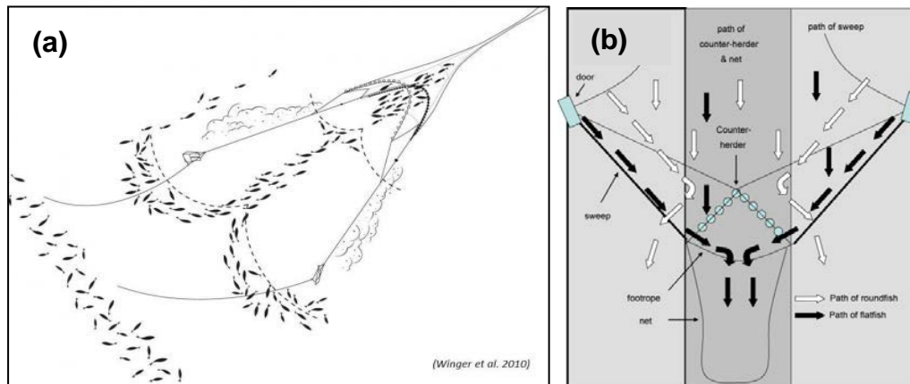
Figure 3. (a) Schematic illustration of the herding process for roundfish species (Winger et al., 2010); (b) Hypothetical floating counter-herding device from Ryer (2008)
