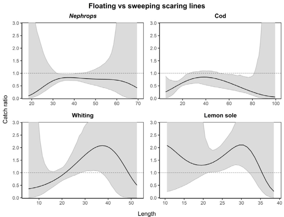
Figure 12. Comparison of FLEXSELECT designs: floating scaring lines (current design) vs sweeping ones (Melli et al., 2018). The curve (solid line) represents the modelled ratio of catch ratio curves from the two individual experiments. The grey ribbon represents 95% CI's estimated from the two bootstrap sets from each catch ratio model estimated for either FLEXSELECT design. The dashed horizontal line, located at 1.0, describes equivalence in efficiency between the FLEXSELECT designs.
